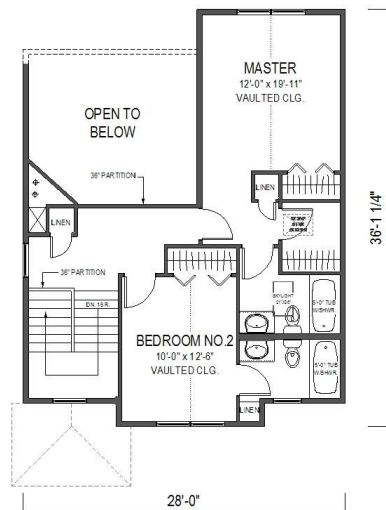
Upper Floor
